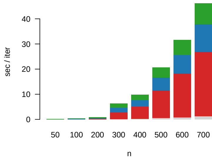
NEW (R=25, fast cov + pivoted Cholesky)
