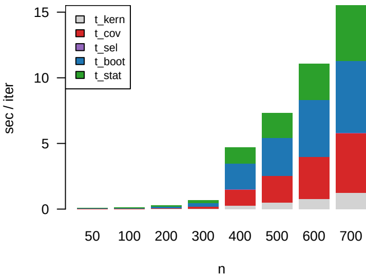
NEW (R=13, fast cov + pivoted Cholesky)
